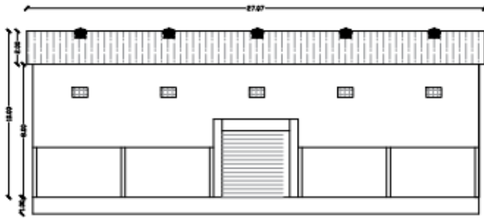
ELEVATION SCALE 1:100
