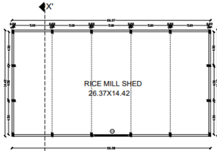
PROPOSED RICE MILL SHED PLAN SCALE 1:100
